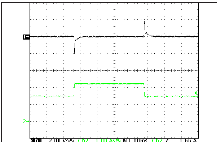
Figure 5: Output voltage response in the QT version to step-change in load current (50% - 75% - 50% of I out (max); dI/dt = 0.1 A/μs). Load cap: 15 μF tantalum cap and 1 μF ceramic cap. Ch 1: V out 2 V/div, Ch 2: I out 1 A/div.
