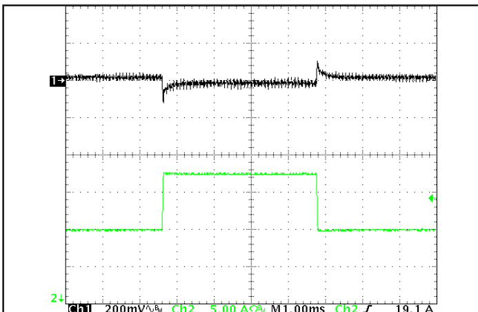
Figure 5: Output voltage response in the QT version to step-change in load current (50% - 75% - 50% of I out (max); dI/dt = 0.1 A/μs). Load cap: 15 μF tantalum cap and 1 μF ceramic cap. Ch 1: V out 200 mV/div, Ch 2: I out 5 A/div.
