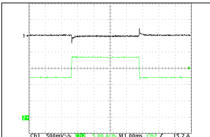
Figure 5: Output voltage response in the QT version to step-change in load current (50 % - 75 % - 50 % of I out (max); dI/dt = 0.1 A/μs). Load cap: 15 μF tantalum cap and 1 μF ceramic cap. Ch 1: V out 500 mV/div, Ch 2: I out 5 A/div.
