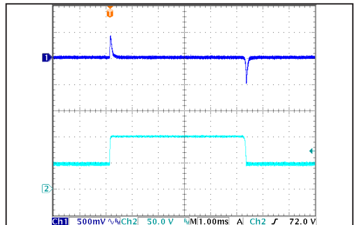
Figure 6: Output voltage response in the QT version to step-change in input voltage (nominal to maximum input voltage), at full load current. Load cap: 1 μF ceramic cap. Ch 1: V out , Ch 2: V in .
