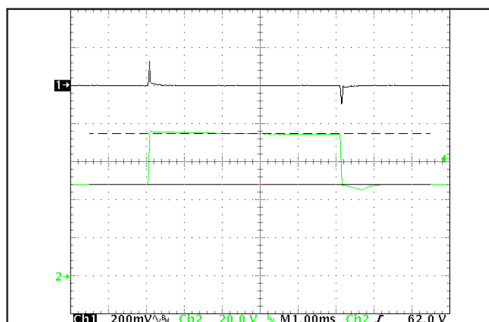
Figure 6: Output voltage response in the QT version to step-change in input voltage (nominal to maximum input voltage), at full load current. Load cap: 15 μF tantalum capacitor and 1 uF ceramic cap. Ch 1: V out , Ch 2: V in .
