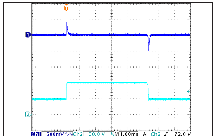
Figure 6: Output voltage response in the QT version to step-change in input voltage (nominal to maximum input voltage), at full load current. Load cap: 15 μF tantalum capacitor and 1 uF ceramic cap. Ch 1: V out , Ch 2: V in .
