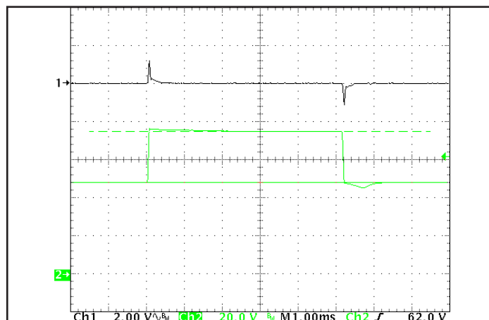
Figure 6: Output voltage response in the QT version to step-change in input voltage (nominal to maximum input voltage), at full load current. Load cap: 1 μF ceramic cap. Ch 1: V out , Ch 2: V in .
