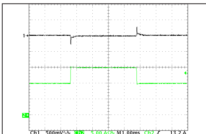
Figure 5: Output voltage response in the QT version to step-change in load current (50 % - 75 % - 50 % of I out (max); dI/dt = 0.1 A/μs). Load cap: 15 μF tantalum cap and 1 μF ceramic cap. Ch 1: V out 500 mV/div, Ch 2: I out 5 A/div.
