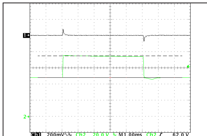
Figure 6: Output voltage response in the QT version to step-change in input voltage (nominal to maximum input voltage), at full load current. Load cap: 15 μF tantalum capacitor and 1 μF ceramic cap. Ch 1: V out , Ch 2: V in .
