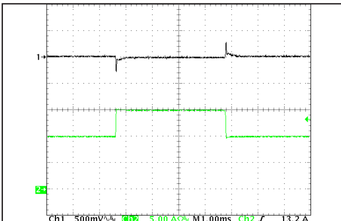
Figure 5: Output voltage response in the QT version to step-change in load current (50% - 75% - 50% of I out (max); dI/dt = 0.1 A/μs). Load cap: 15 μF tantalum cap and 1 μF ceramic cap. Ch 1: V out 500 mV/div, Ch 2: I out 5 A/div.
