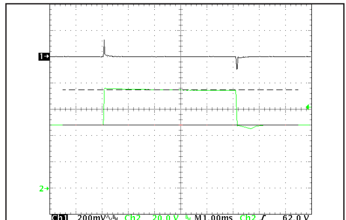
Figure 6: Output voltage response in the QT version to step-change in input voltage (nominal to maximum input voltage), at full load current. Load cap: 15 μF tantalum capacitor and 1 μF ceramic cap. Ch 1: V out , Ch 2: V in .
