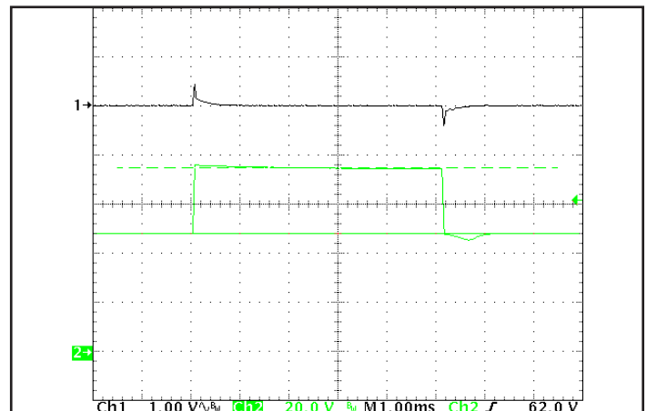
Figure 6: Output voltage response in the QT version to step-change in input voltage (nominal to maximum input voltage), at full load current. Load cap: 1 \mu F ceramic cap. Ch 1: V_{out} , Ch 2: V_{in} .
